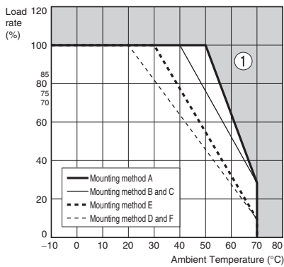
Mounting method A (Standard mounting method)
